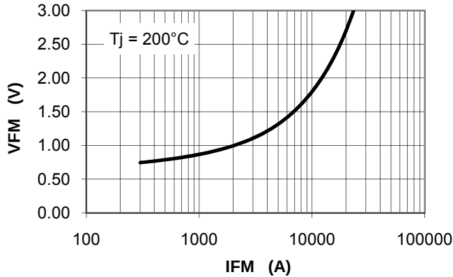
Maximum On-State Voltage Drop
