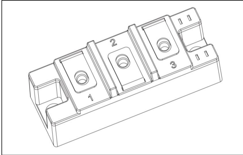
Dual SiC Diode Module 100 Amperes / 3300 Volts
